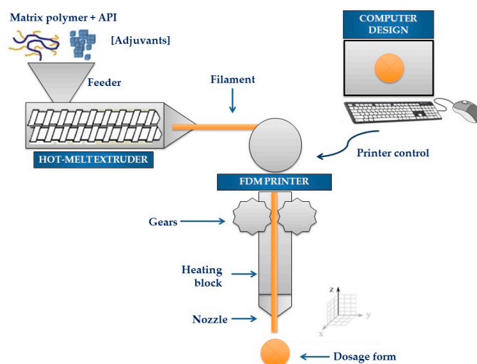
Figure 3. Schematic representation of integrated hot-melt extrusion and fused deposition modelling for pharmaceutical applications.
