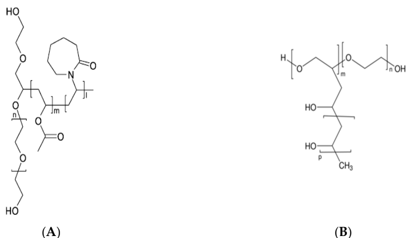
Figure 10. Chemical structure of (A) Soluplus ® [79] and (B) Kollicoat ® IR [79].
