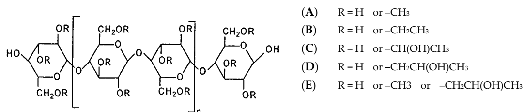
Figure 6. Chemical structure of cellulose ethers derivatives—methylcellulose (A), ethylcellulose (B), hydroxyethylcellulose (C), hydroxypropylcellulose (D), and hydroxypropylmethylcellulose (E).
