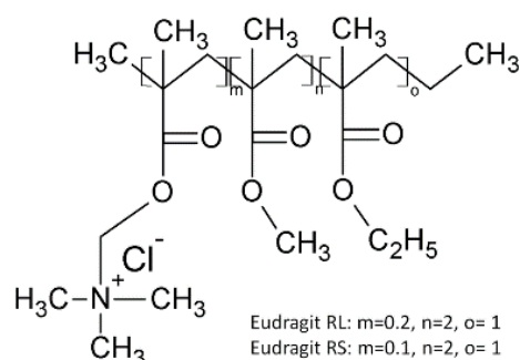
Figure 9. Chemical structure of Eudragit ® RL and RS [114].
