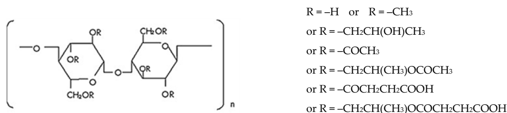
Figure 7. Chemical structure of hydroxypropylmethylcellulose acetate succinate [34,35].
