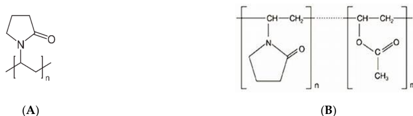
Figure 5. Chemical structure of water-soluble polyvidone (PVP) (povidone; (A)) and water-insoluble PVP vinyl acetate copolymer (copovidone; (B)).
