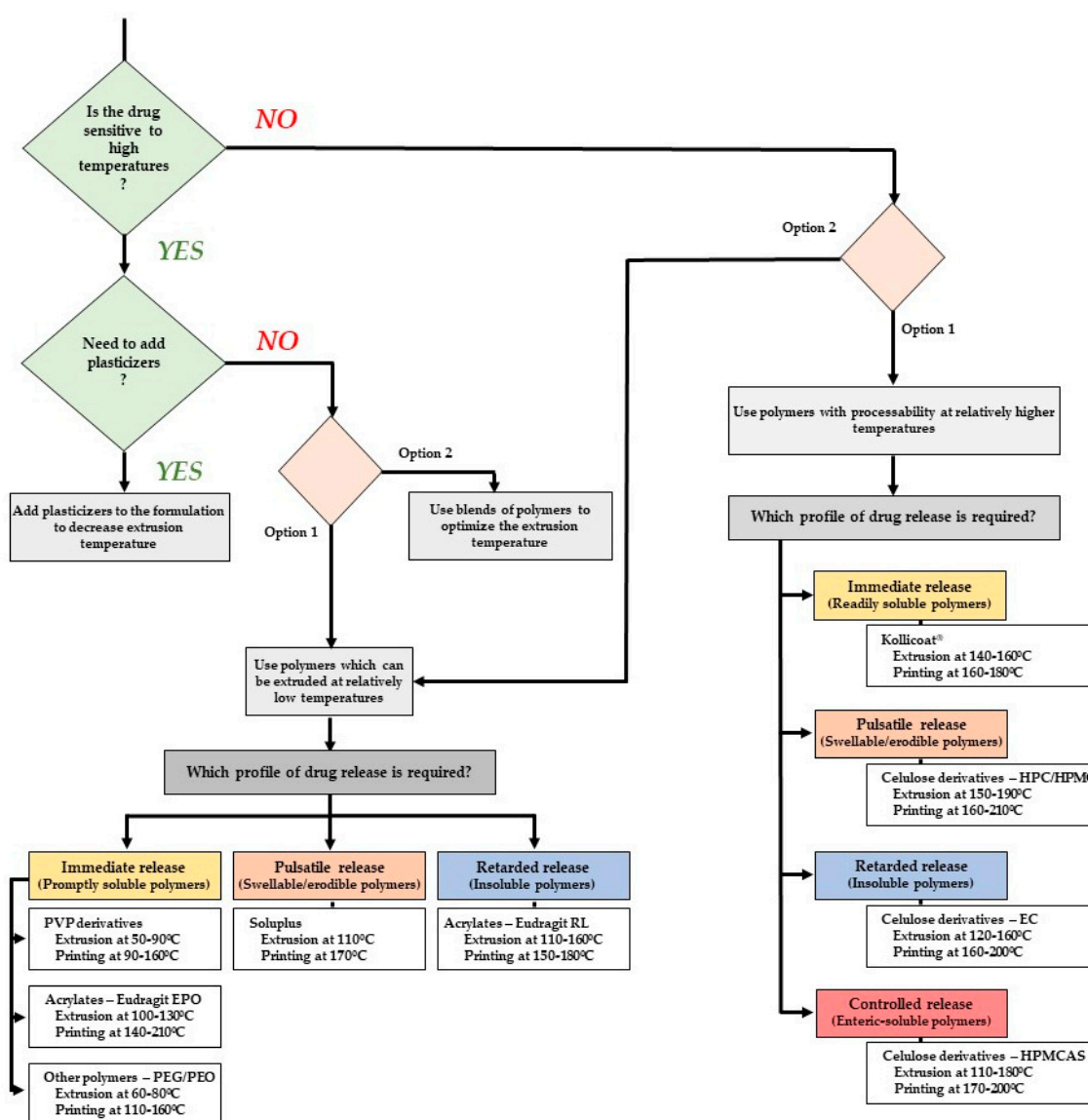
Figure 13. Decision tree for the choice of a polymer for HME coupled to FDM, considering drug thermal sensitivity, impact of thermal properties of the polymer on extrudability/printability, and desired drug release profile.
