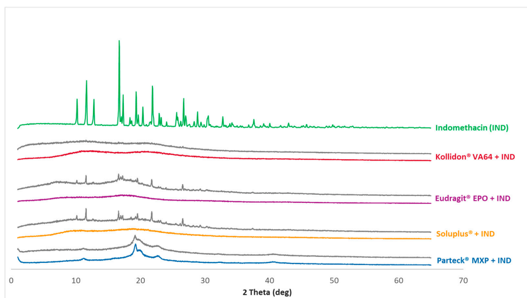
Figure 5. PXRD measurements: The curves for the formulations are clustered. In front of each cluster are the VCM-processed samples with a color code used throughout the data; and in the back are the cryo-milled physical mixtures for each polymer and indomethacin depicted in gray. A pure indomethacin diffractogram for reference purpose is given in the back as a single curve.
