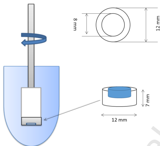
Figure 1 technical diagram of the new fabricated dies and die assembly for the IDR testing
