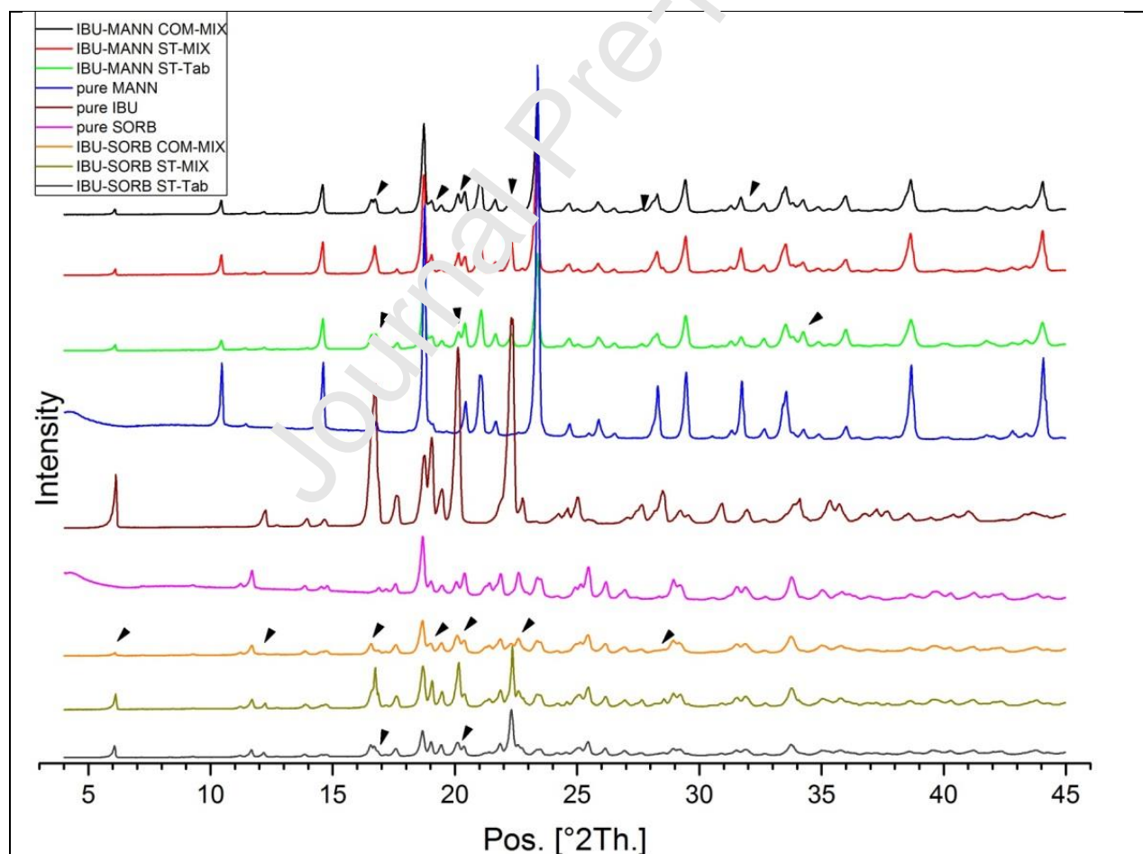
Figure 6 XRPD patterns of standard tablets and co-milled mixtures as compared to standard physical mixtures: IBU-MANN, IBU-SORB and the pure compounds.
