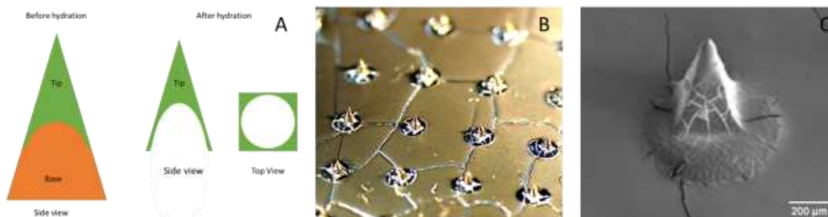
Figure 2. A) Schematic representation of the needle in this study, before and after hydration, as shown by CARS and multiphoton excitation microscopy. To the left shows the needle from the side, which is divided into a base and a tip, the latter which contains the active substance. To the right is the top view of the needle. B) Image showing a part of the patch with 49 needles. C) SEM image of a characteristic microneedle.
