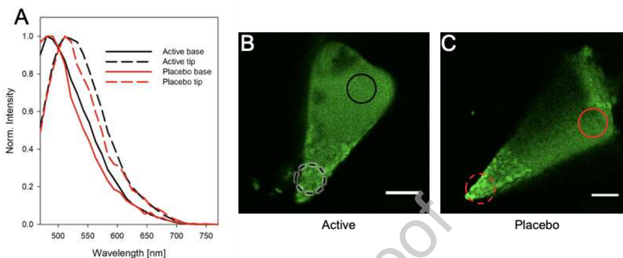
Figure 3. Emission spectra of a placebo and active needle. A) Emission spectrum with the normalized intensity as function of wavelength [nm] for the tip of a placebo needle (dashed red); the base of a placebo needle (solid red); the tip of an active needle (dashed black) and the base of an active needle (solid black). B) A fluorescence image of an active needle showing where the emission was measured for the tip of the needle (dashed circle) and the base of the needle (solid circle). Scalebar is 100 \mu\text{m} . C) A fluorescence image of a placebo needle showing where the emission was measured for the tip of the needle (dashed circle) and the base of the needle (solid circle). Scalebar is 100 \mu\text{m} .
