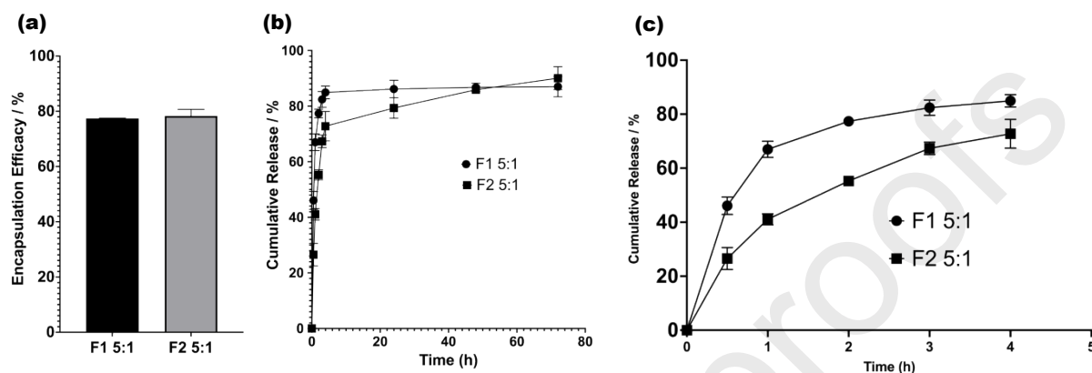
Figure 5. (a) Encapsulation Efficiency for F1 and F2, using 1 mg/ml AMOX and a 5:1 FRR and (b) 72-hour release profiles for F1 and F2, using 1 mg/ml AMOX and a 5:1 FRR and (c) A detailed portrayal of the burst release exhibited in the first 4 hours by F1 and F2.
