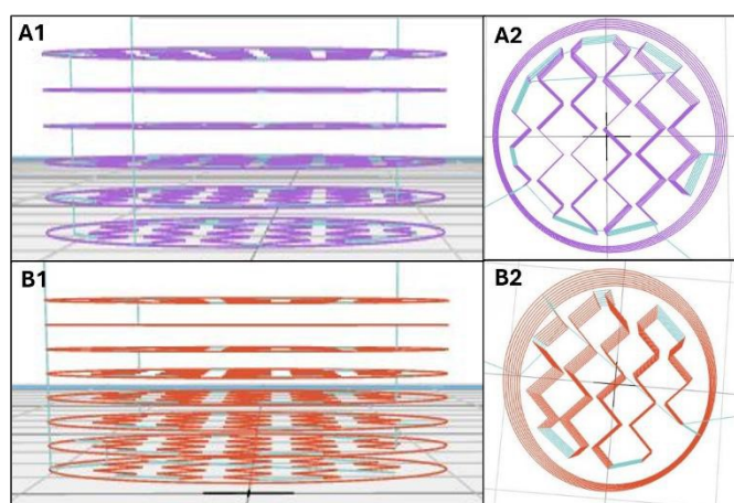
Fig. 1 Computer-aided designs were sliced before 3D printing. A1) and B1) show the lateral view of the IR and ER layers. A2) and B2) show the top view of each tablet layer.
