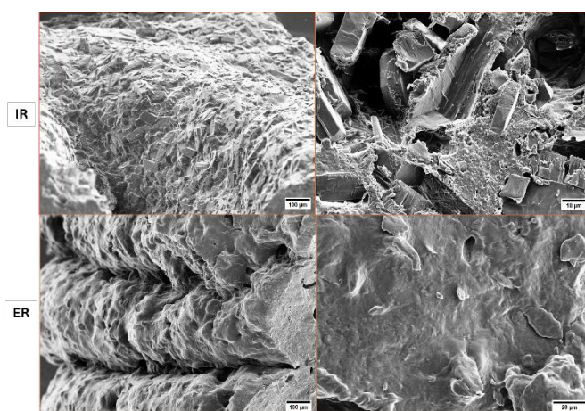
Fig. 5 The left side shows SEM images of the dual-release drug-loaded tablet surface area of immediate (IR) and a lateral view of ER.
