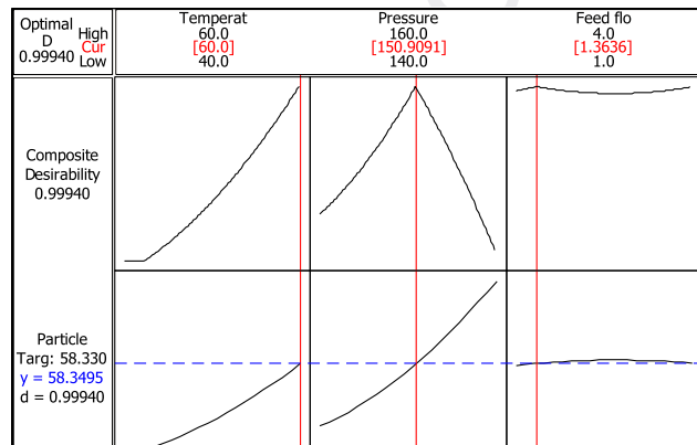
Figure 4 – Response optimizer at the optimum condition for target goal.
