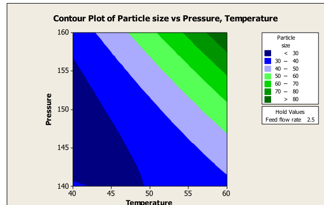
Figure 5 – Response contour plot of particle size ( \mu\text{m} ) at a feasible optimum condition.
