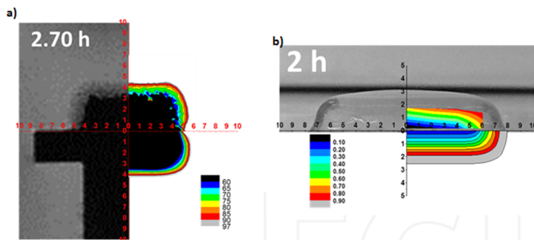
Figure 7. a) On the left, NMR image of a swollen matrix composed of HPMC after 2.7 h of dissolution. At the top, experimental water fraction distribution; at the bottom, calculated water fraction distribution. b) On the left top, photo of a semioverall system after 2 h of dissolution (the matrix was cut along its diameter). On the right top, experimental water mass fraction obtained by texture analysis; on the bottom right, model predictions. In both images, the dimensions are in mm; the color scale is referred to the water content fraction (black = lower water content; gray = fully hydrated matrix).
