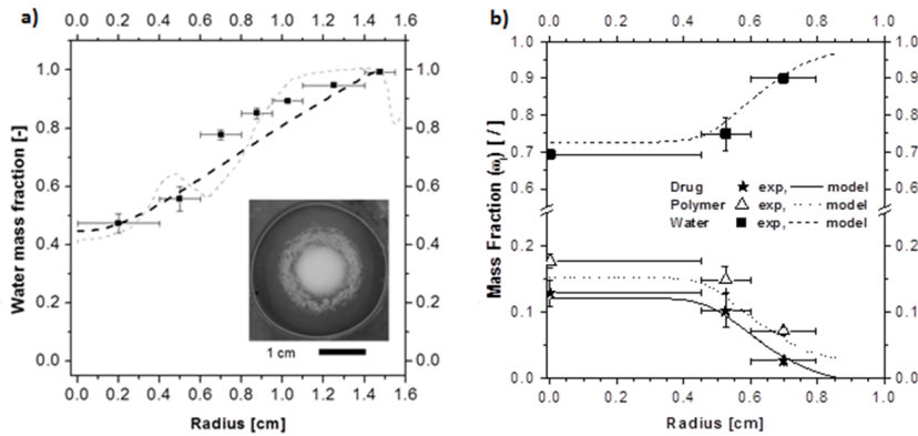
Figure 5. a) Water mass fraction along the radial direction after 48 h of dissolution of a radial system. The full squares are the experimental data obtained by the gravimetric analysis; the dotted gray curve is the result of the image analysis; the dashed black curve is the model prediction. In the inset, the real photo of the matrix used for the image analysis. b) Mass fraction evolutions along the radial direction for semioverall system after 6 h of dissolution (the values are averaged along the thickness direction). The scatters are the experimental data; the curves are the model predictions. In both the graphs, the vertical bars represent the standard deviation between the experimental runs, and the horizontal bars represent the extension of the section cut by the punch.
