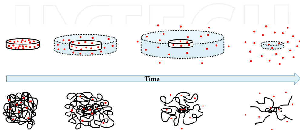
Figure 2. Drug release from a matrix (tablet) made of swellable hydrogel. The phenomena (described in the text) of water uptake, swelling, polymer chain relaxation, drug diffusion, polymer chain disentanglement, and polymer erosion are graphically depicted.
