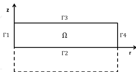
Figure 11. Computational domain for the model of Caccavo et al. [114, 115]
