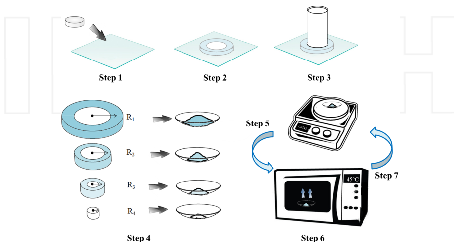
Figure 6. Experimental procedure used to evaluate the mass evolutions inside a swollen matrix by gravimetric technique.
