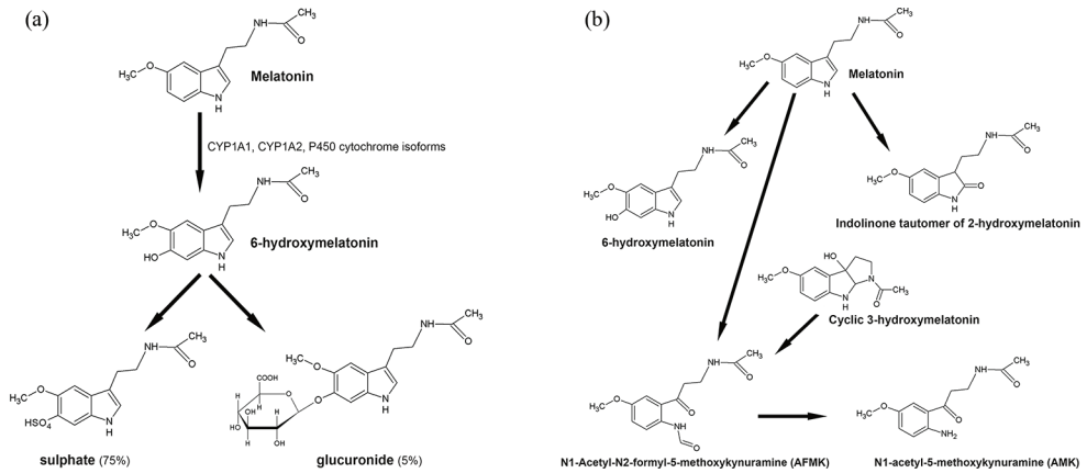
Figure 3. Melatonin hepatic (a) and cerebral (b) metabolism.
