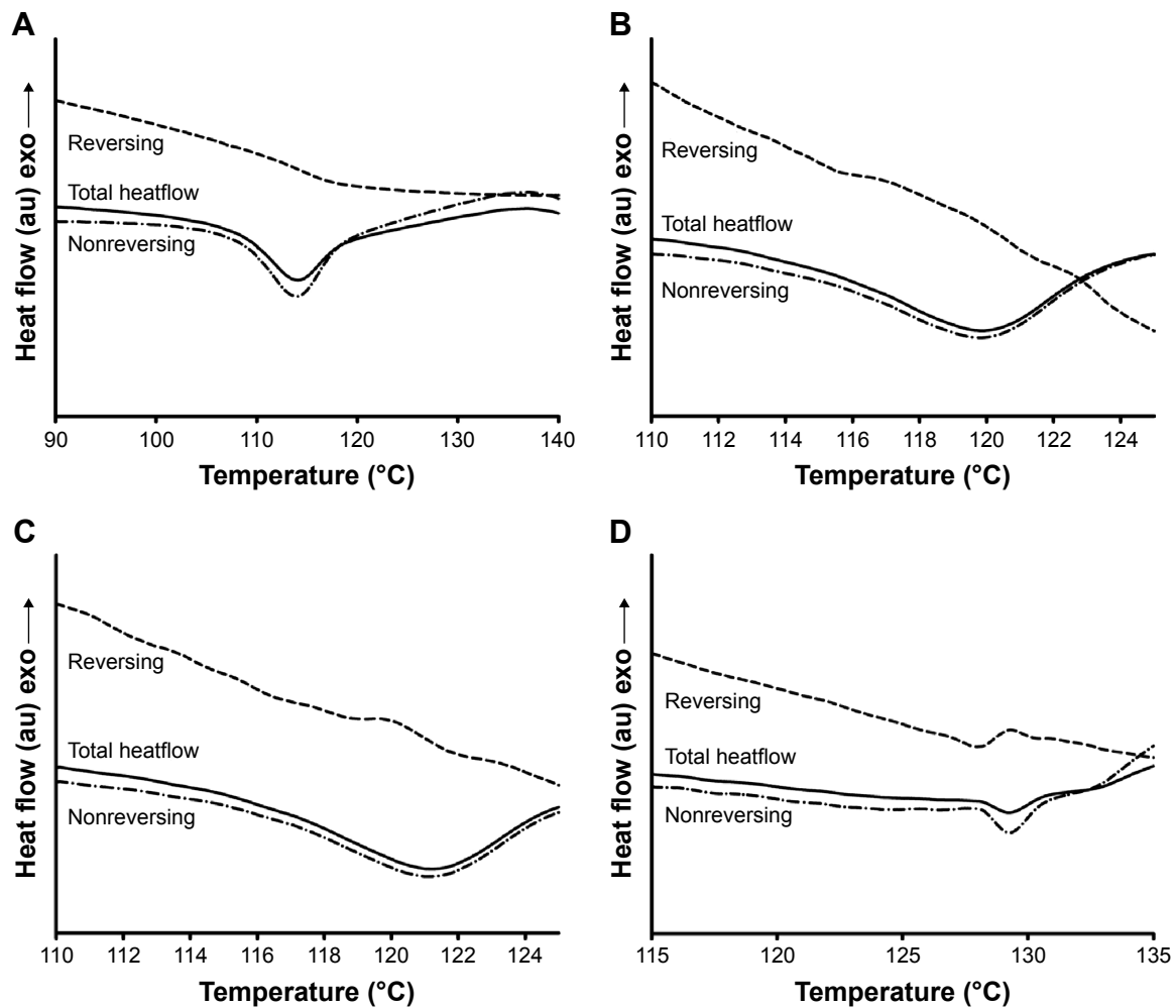
Figure S1 DSC thermograms of BSA and freeze-dried cakes. Notes: (A) BSA; (B) BSA + 1% sucrose; (C) BSA + 1% trehalose; (D) BSA + 1% aminoclay. Abbreviation: BSA, bovine serum albumin.
