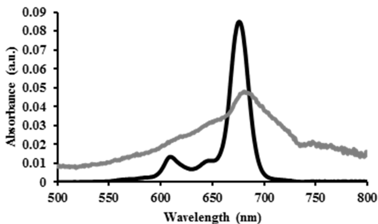
Figure 3. UV-VIS spectra of AlCIPc molecules (black) and AlCIPc-MSNs (gray).
